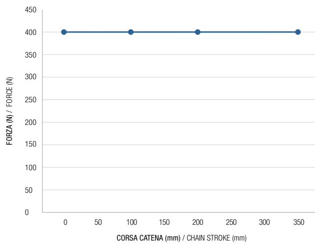
L40 Slim - 350 - Portate attuatori vasistas L40 Slim - 350 - Actuator force - bottom hung
