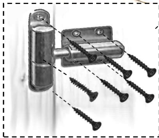
OUTSIDE \varnothing 3,5 \times 35 (x7)
